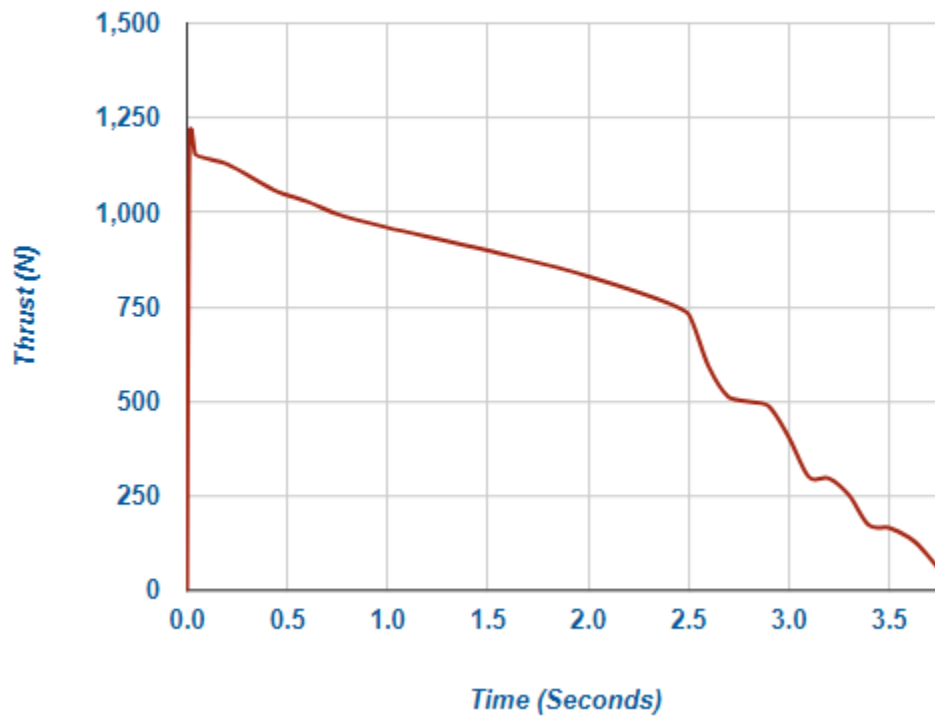
Figure 3.3.1.2. Thrust vs Time
