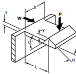
Figure 5.1.1.4. Geometric Relations to Variables
