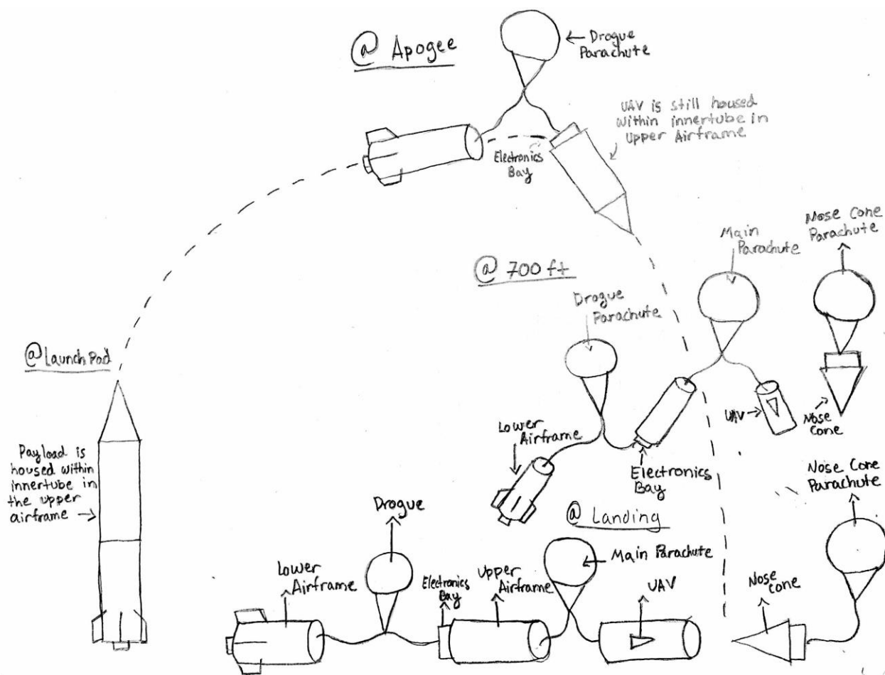
Figure 3.2.1. Flight Plan
