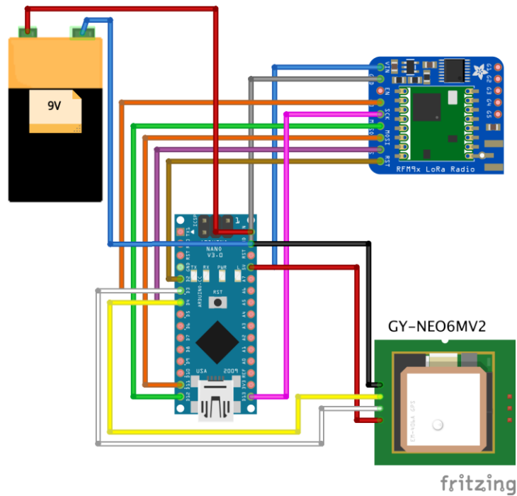
Figure 3.4.2.1. GPS Circuit Diagram
